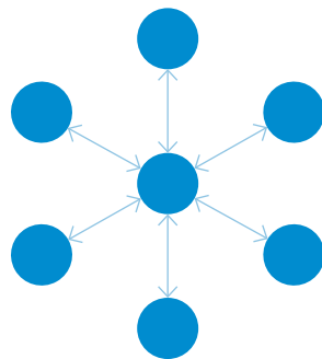
a) Centralized
