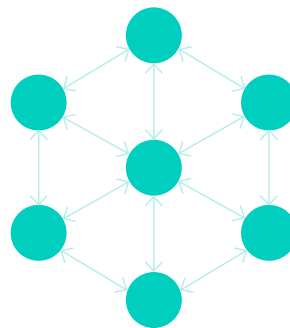
b) Federated
